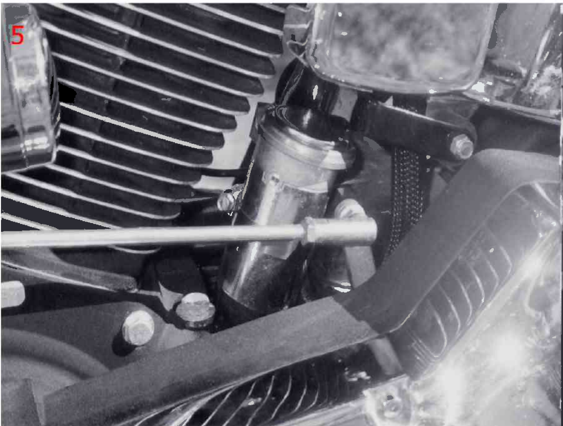
Photo (5) shows the location on most Softtail models, attached to the frame tube behind the rear cylinder using a #40 hose clamp not provided. When tightening the hose clamp maintain at least 1/4" clearance between the compressor, rear cylinder and the shift linkage.
